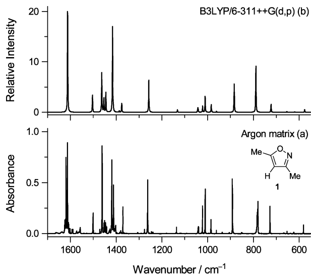
Figure 1. (a) Experimental FTIR spectrum of 3,5-dimethylisoxazole ( 1 ) isolated in an argon matrix at 15 K. (b) IR spectrum of 1 simulated at the B3LYP/6-311++G(d,p) level of theory (for details, see the Experimental Section).
