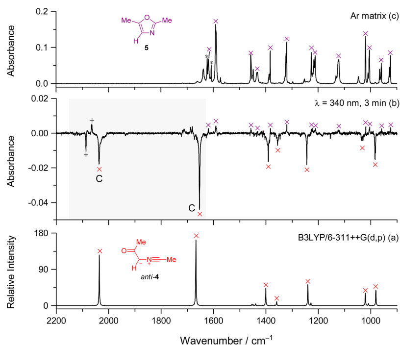
Figure 5. (a) IR spectrum of nitrile ylide anti - 4 simulated at the B3LYP/6-311++G(d,p) level. (b) Experimental difference IR spectrum showing changes after 3 min of UV irradiation at \lambda = 340 nm (subsequent to 80 min of irradiation at \lambda = 222 nm). Growing bands are displayed upward. The violet crosses (X) designate the bands formed at the expense of C and assigned to 2,5-dimethyloxazole ( 5 ) (positive bands). The red crosses (X) designate the bands of C assigned to anti - 4 (negative bands). The plus signs (+) indicate bands due to photoproduct B , as assigned in Figure 4. (c) Experimental IR spectrum of authentic 2,5-dimethyloxazole ( 5 ) isolated in an argon matrix in a separate experiment. 25 The asterisks (*) indicate bands of monomeric water.
