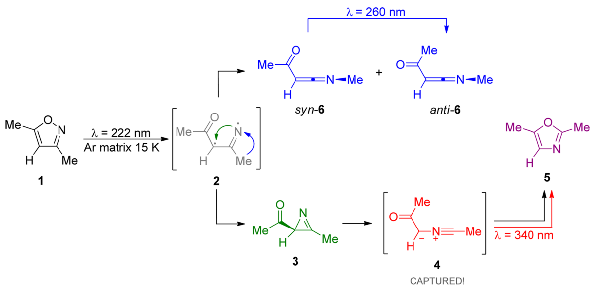
Scheme 2. Summary of the Experimental Observations and the Mechanism for Photochemistry of 3,5-Dimethylisoxazole 1 Isolated in a Low-Temperature Argon Matrix
