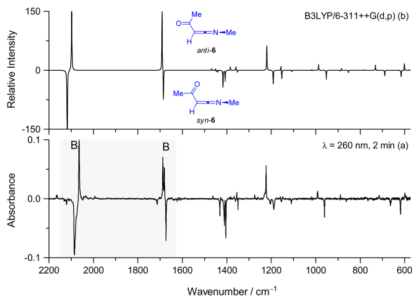
Figure 4. (a) Experimental difference IR spectrum showing changes in the spectrum of photoproduct B after 2 min of UV irradiation at \lambda = 260 nm (after irradiations at 222 nm and at 340 nm). Growing bands are displayed upward. (b) IR spectrum simulated at the B3LYP/6-311++G(d,p) level considering the consumption of syn -3-acetyl- N -methylketenimine ( syn - 6 ) and the production of anti -3-acetyl- N -methylketenimine ( anti - 6 ).
